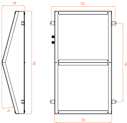
M01: Surface Mounting
