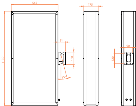
M01: Surface Mounting
